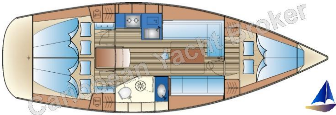
Layout / Bavaria 35 Cruiser - 2010
