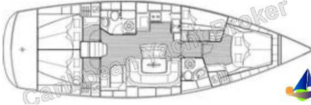
Layout / Bavaria - 46 Cruiser / 2008
